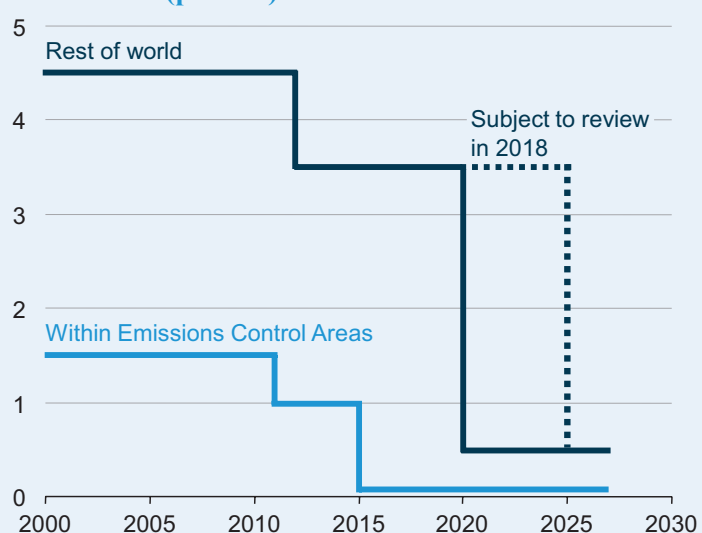
Figure 2-6. Current and proposed Marpol regulations on sulfur content of residual fuel oil, 2000–2027 (percent)
