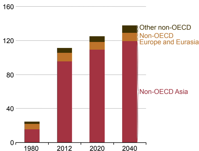
Figure 4-6. Non-OECD coal consumption by region, 1980, 2012, 2020, and 2040 (quadrillion Btu)
