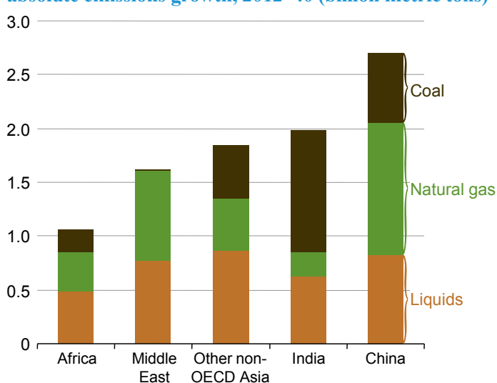
Figure 9-7. Increases in carbon dioxide emissions by fuel type in non-OECD regions with the highest absolute emissions growth, 2012–40 (billion metric tons)
